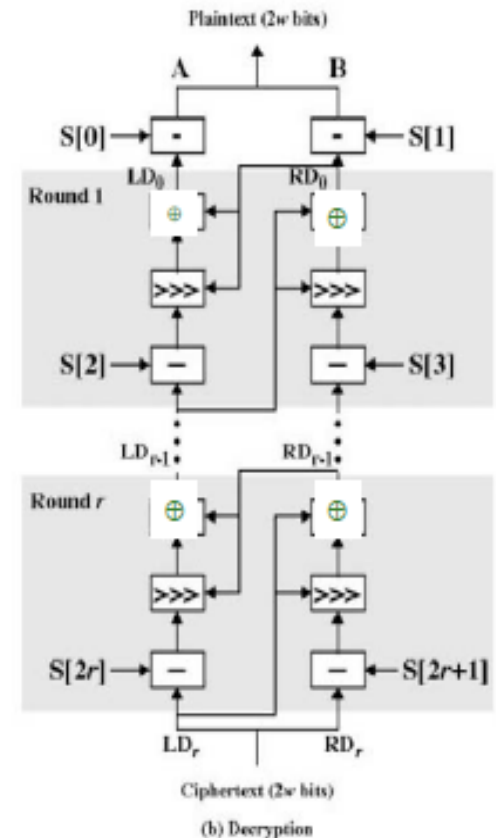
Figure 6.6 RC5 Encryption and Decryption
