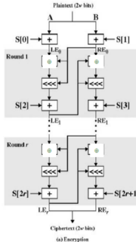
Figure 6.6 RC5 Encryption and Decryption
